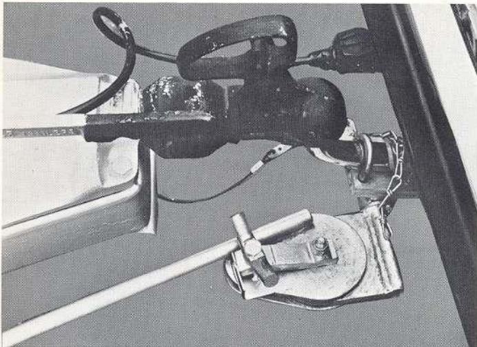
Caravan stabilisator. 9627.19
